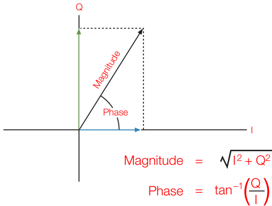
Figure 2-33. Vector representation of magnitude and phase.
