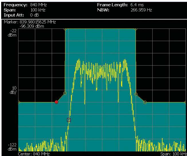
Figure 2-30. Frequency mask definition.
