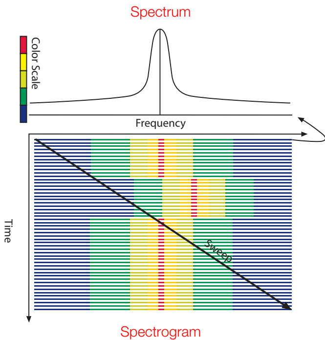
Figure 2-6. Spectrum, Spectrogram and Sweep.
