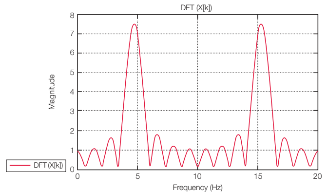
Figure 2-12. DFT of x(n) evaluated continuously.
