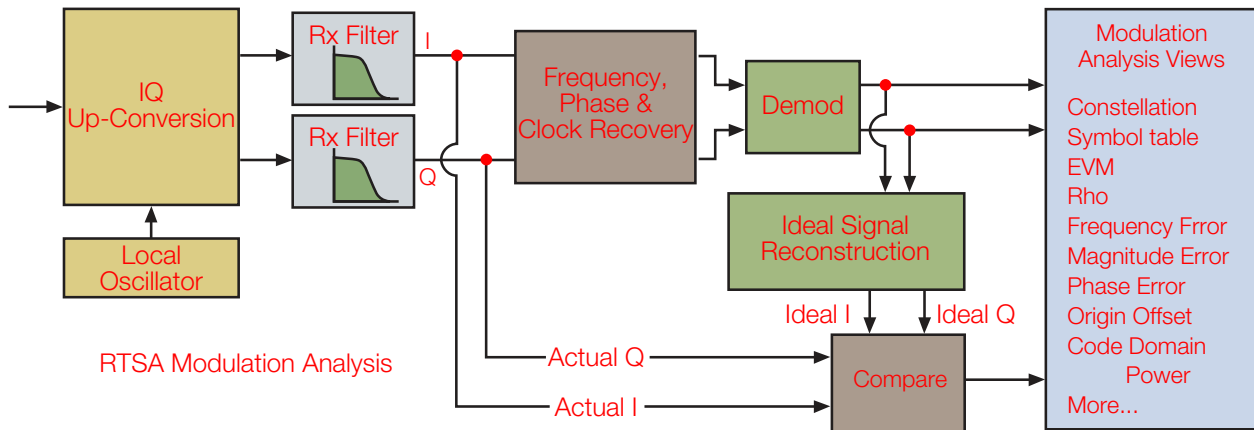
Figure 2-35. RTSA modulation analysis block diagram.
