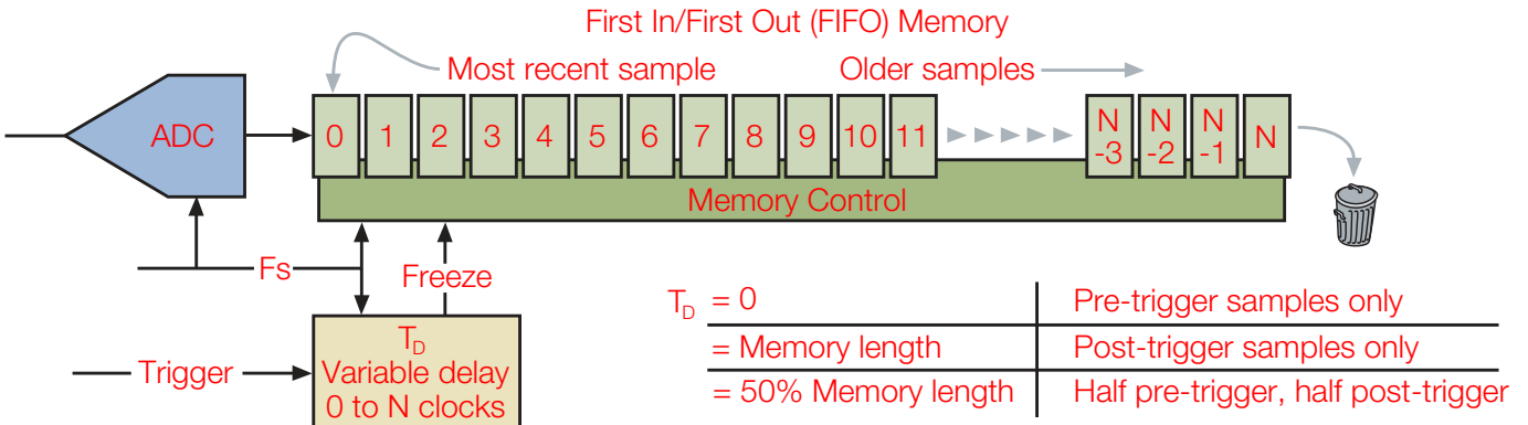
Figure 2-28. Triggering in digital acquisition systems.
