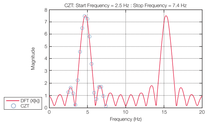
Figure 2-14. CZT of x(n) .
