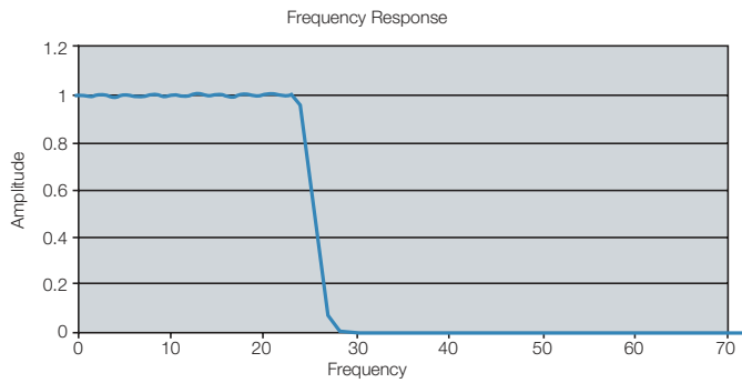
Figure 2-15. Frequency response of a lowpass filter.
