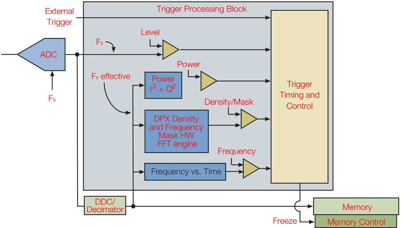
Figure 2-29. Real-Time Spectrum Analyzer trigger processing.
