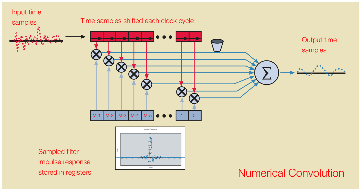
Figure 2-19. Discrete Time Numerical Convolution.
