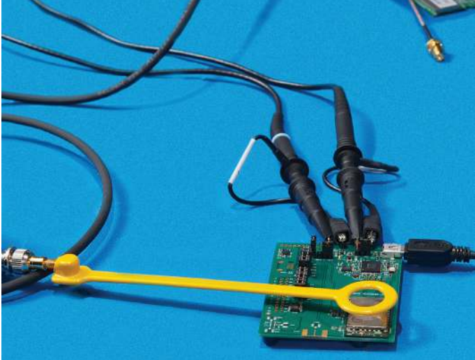
Figure 16. A near field probe can be used to discover the location of unintended RF emissions.
