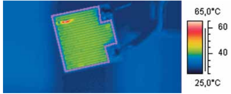
A flawed resistor controlled with a thermal imaging camera
