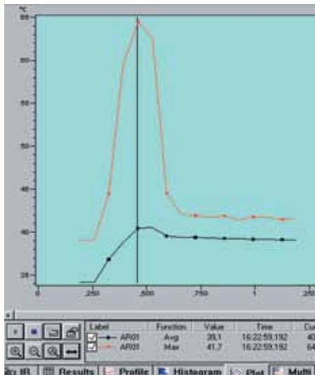
The time trend analysis of the maximum and average temperatures of a faulty component, using the specially developed machine vision software.
