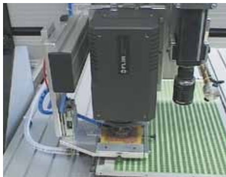
Each component is individually inspected by the FLIR thermal imaging camera.
