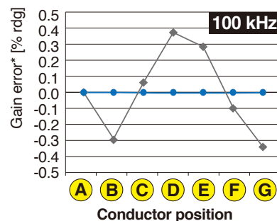
— CT6904A — Sensors designed without accounting for conductor position deviation from center
