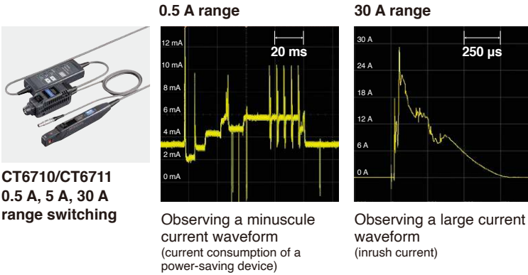
Observing currents of a variety of magnitudes, from minuscule currents to large currents, with a single probe
